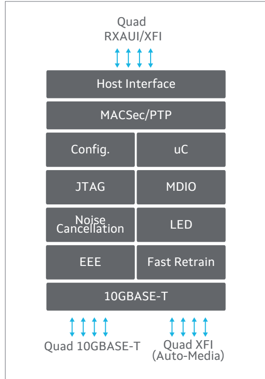
Fig 1. Marvell Alaska X 88X3240P
