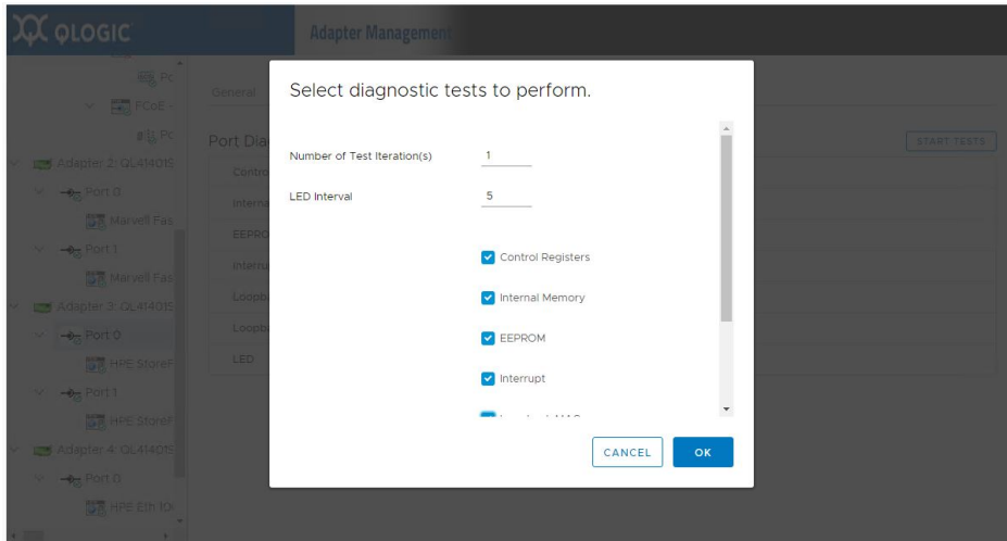
Figure 5-14. Diagnostics Pane
