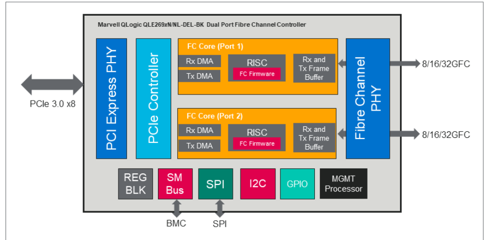
Figure 1. Marvell QLogic 2690 Series Adapters Block Diagram
